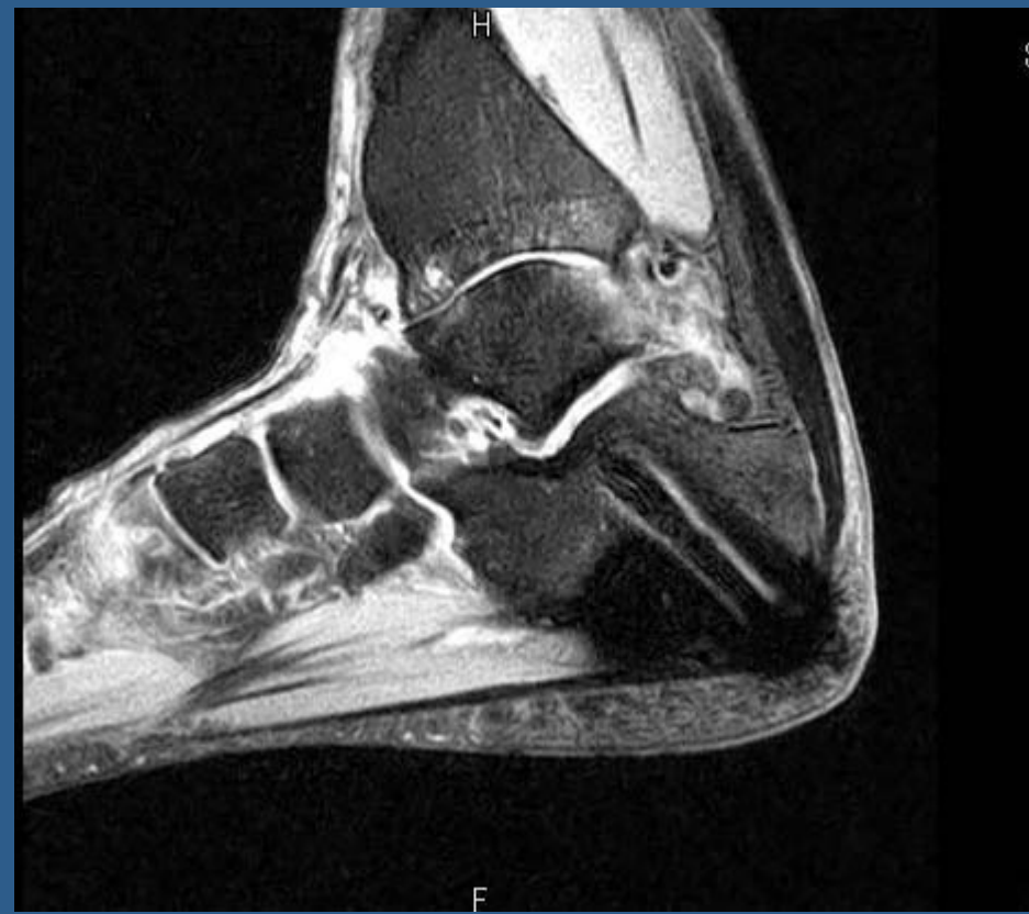
T2 Weighted
