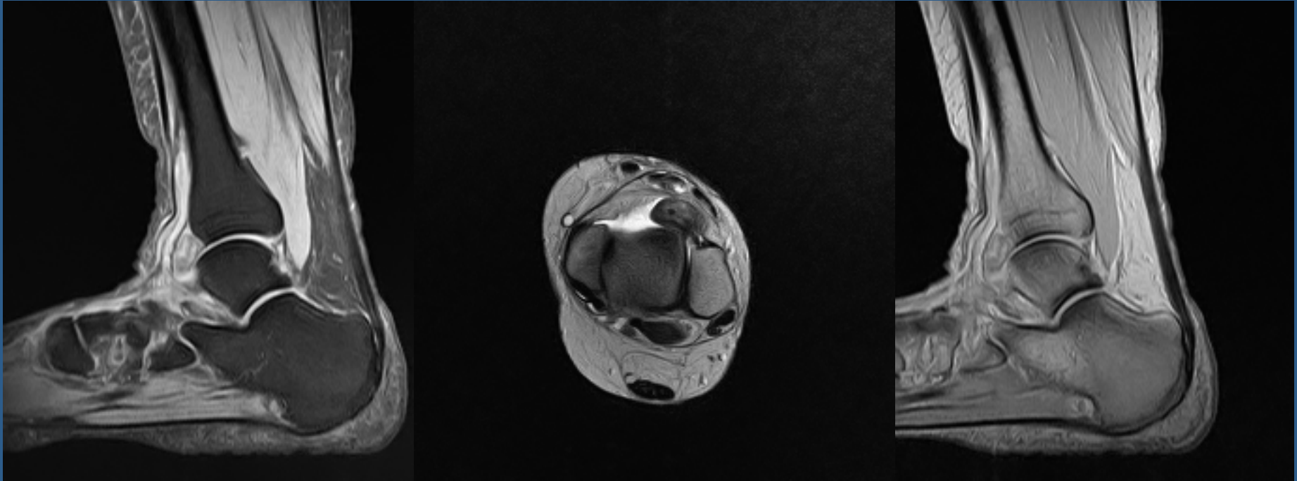
Fat Suppressed
